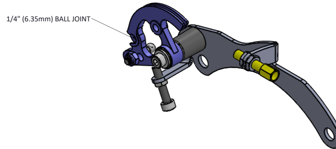
THROTTLE CABLE ADJUSTER
